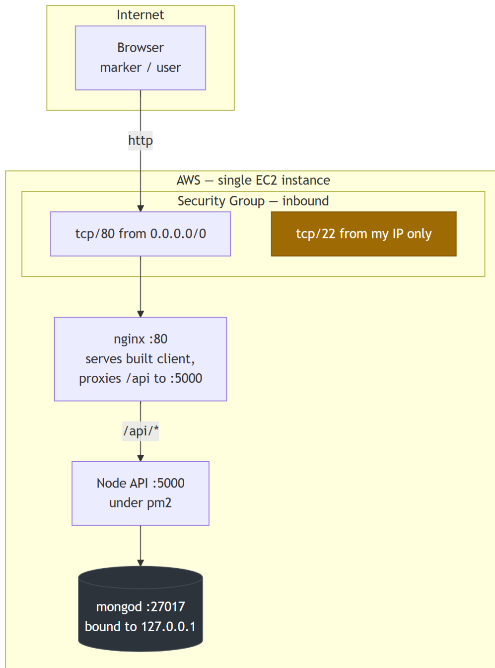
Figure 10. Deployment view. One instance runs the proxy, the API and the database, with only port 80 reachable publicly.
