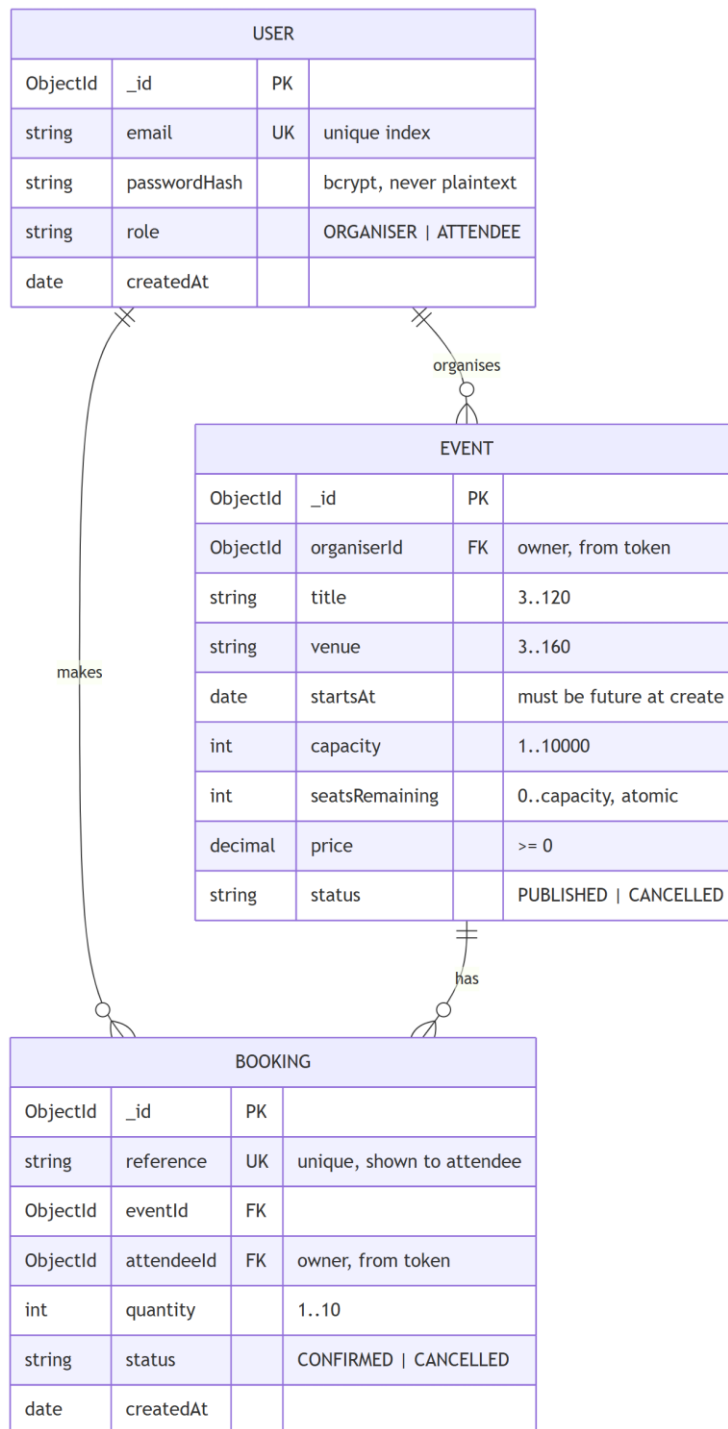
Figure 9. Data model.
